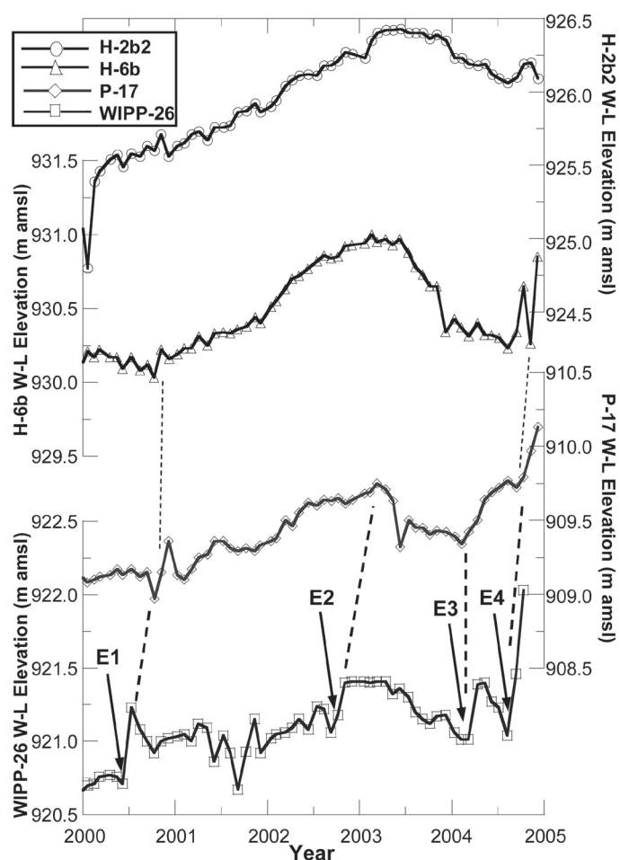
FIGURE 8. Hydrographs, 2000 to 2004, of WIPP-26 located in southern Nash Draw, P-17 south of the WIPP site, H-6b north of the WIPP site, and H-2b2 close to the center of the WIPP site. E# denotes rainfall events listed in Table 2. Dashed lines indicate possible correlation of events. Water level (W-L) is not corrected for density variations and is plotted as an elevation in meters above mean sea level (m amsl).
