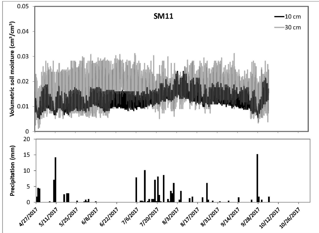
Soil moisture time series for SM11, located close to the cliff under a small overhang. The bottom graph shows local precipitation amounts.
