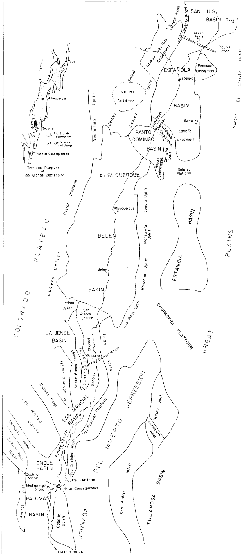
MAP OF A PART OF THE RIO GRANDE DEPRESSION SHOWING MAJOR TECTONIC FEATURES
